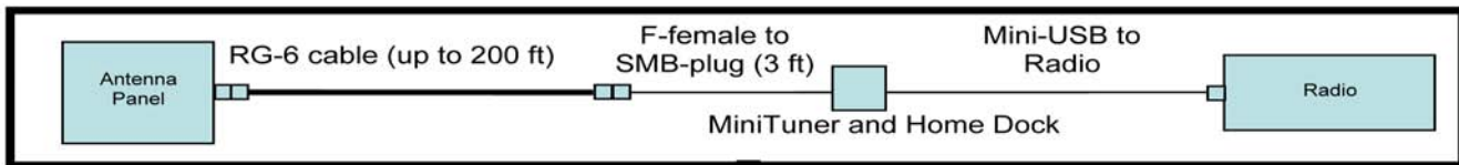
Figure 5: Electrical Connections
