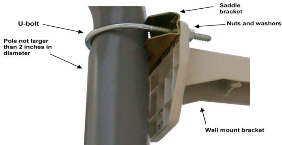
Figure 6: Pole Mount U-bolt & saddle
