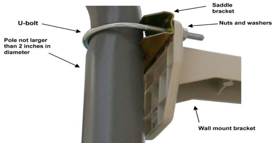
Figure 6: Pole Mount U-bolt & saddle
