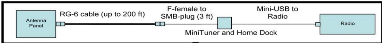
Figure 5: Electrical Connections
