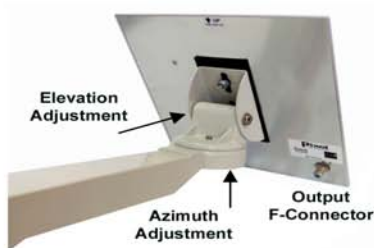
Figure 2: Elevation and Azimuth Adjustments
