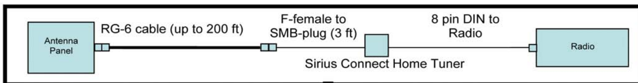
Figure 5: Electrical Connections
