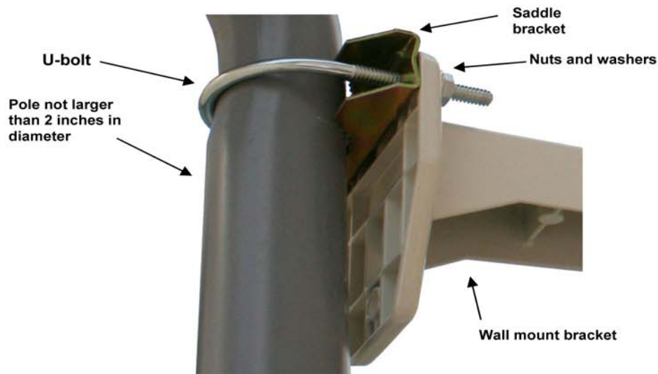
Figure 6: Pole Mount U-bolt & saddle
