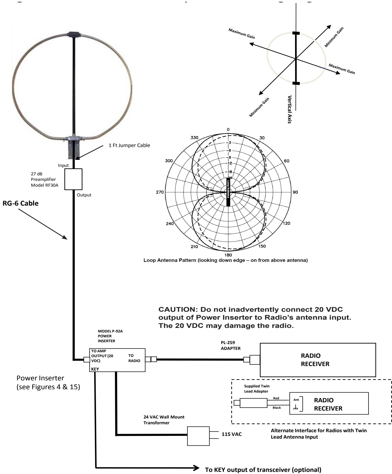
Figure 1. RF PRO-1B Active Loop Antenna Wiring Diagram
