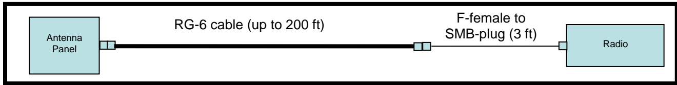
Figure 2: Electrical Connections
